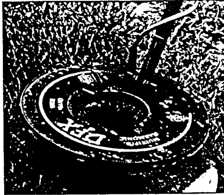
The 9.5in concentric and 10in x 5in elliptical coils used in the test.
